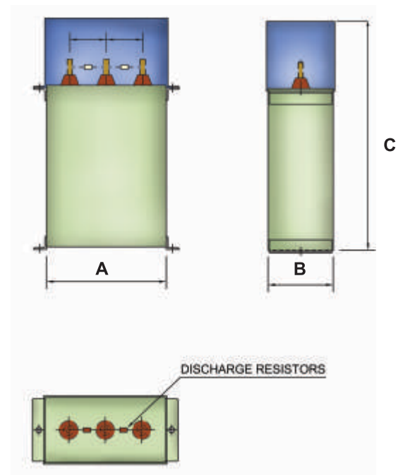
Capacitor Bank
